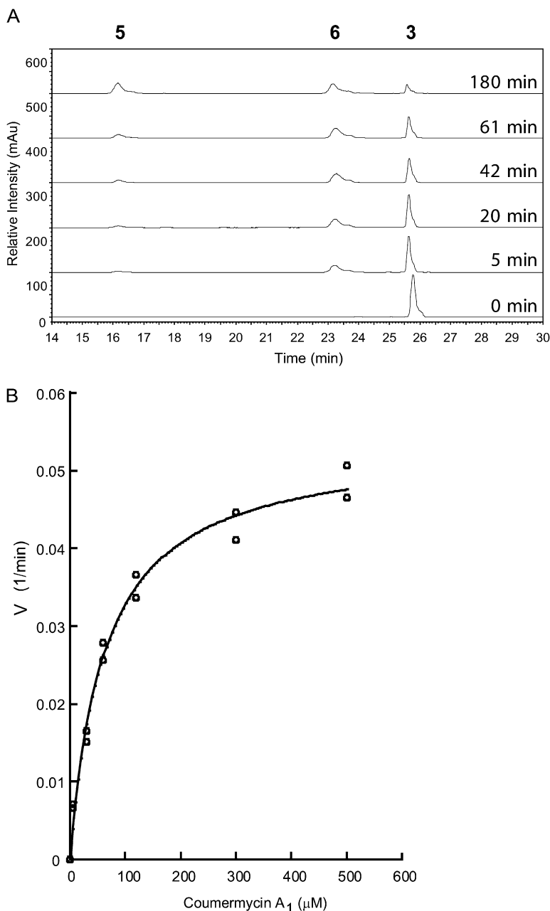
Figure 4. CouN7 Will Deacylate Coumermycin A 1
