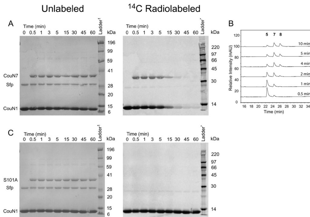
Figure 3. Acylation of Des-5-Methylpyrrolylcoumermycin 5 Proceeds via an Acyl-O-CouN7 Intermediate by Using S 101
